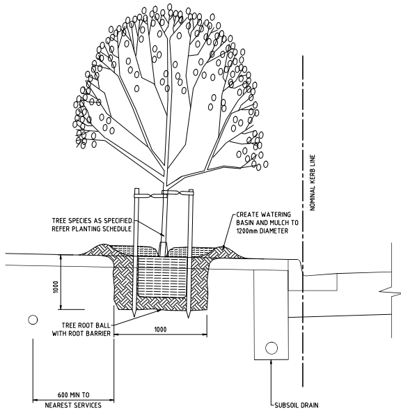
TYPICAL TREE PLANTING BED 1/25
