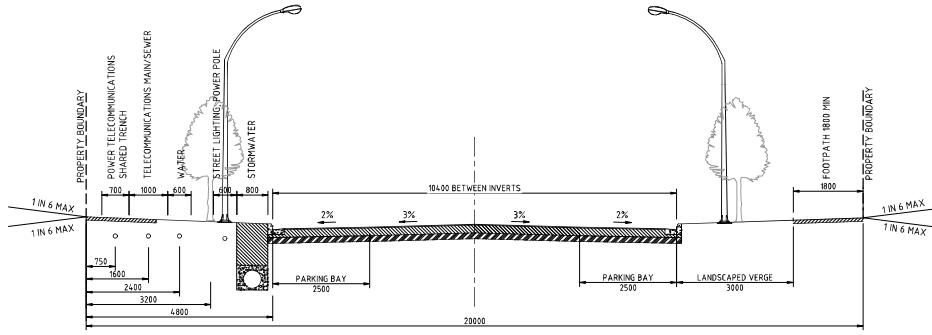
URBAN RESIDENTIAL - COLLECTOR, LOCAL <= 1000m 2 - WITHOUT BULB-OUT SECTION 1:100
