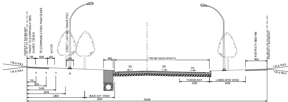
URBAN RESIDENTIAL - COLLECTOR, LOCAL <= 1000m 2 - WITH BULB-OUT SECTION 1:100
